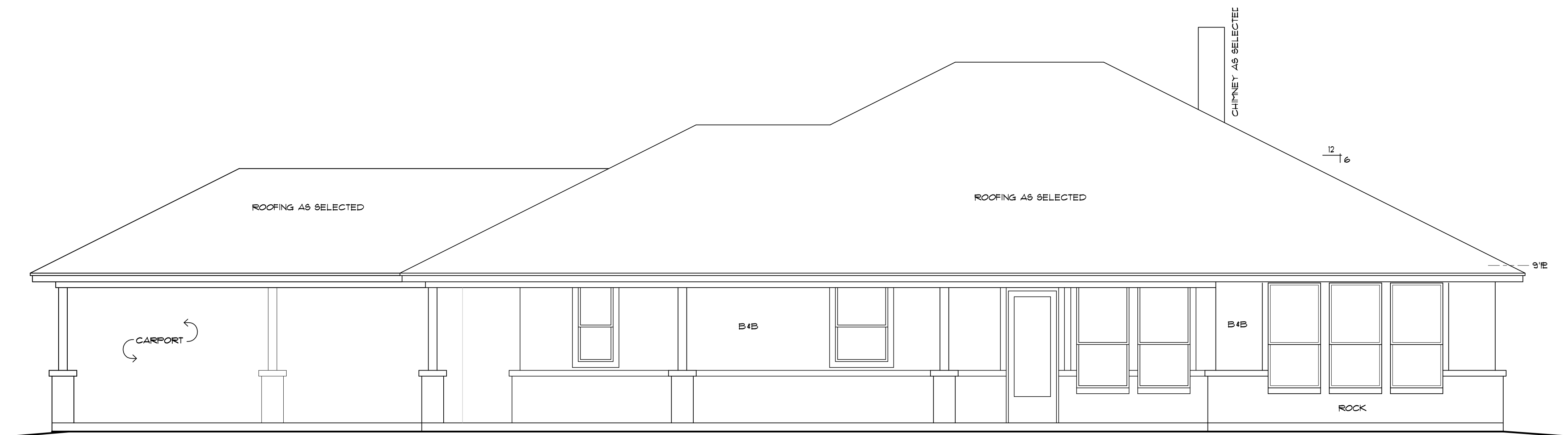
FRONT ELEVATION
